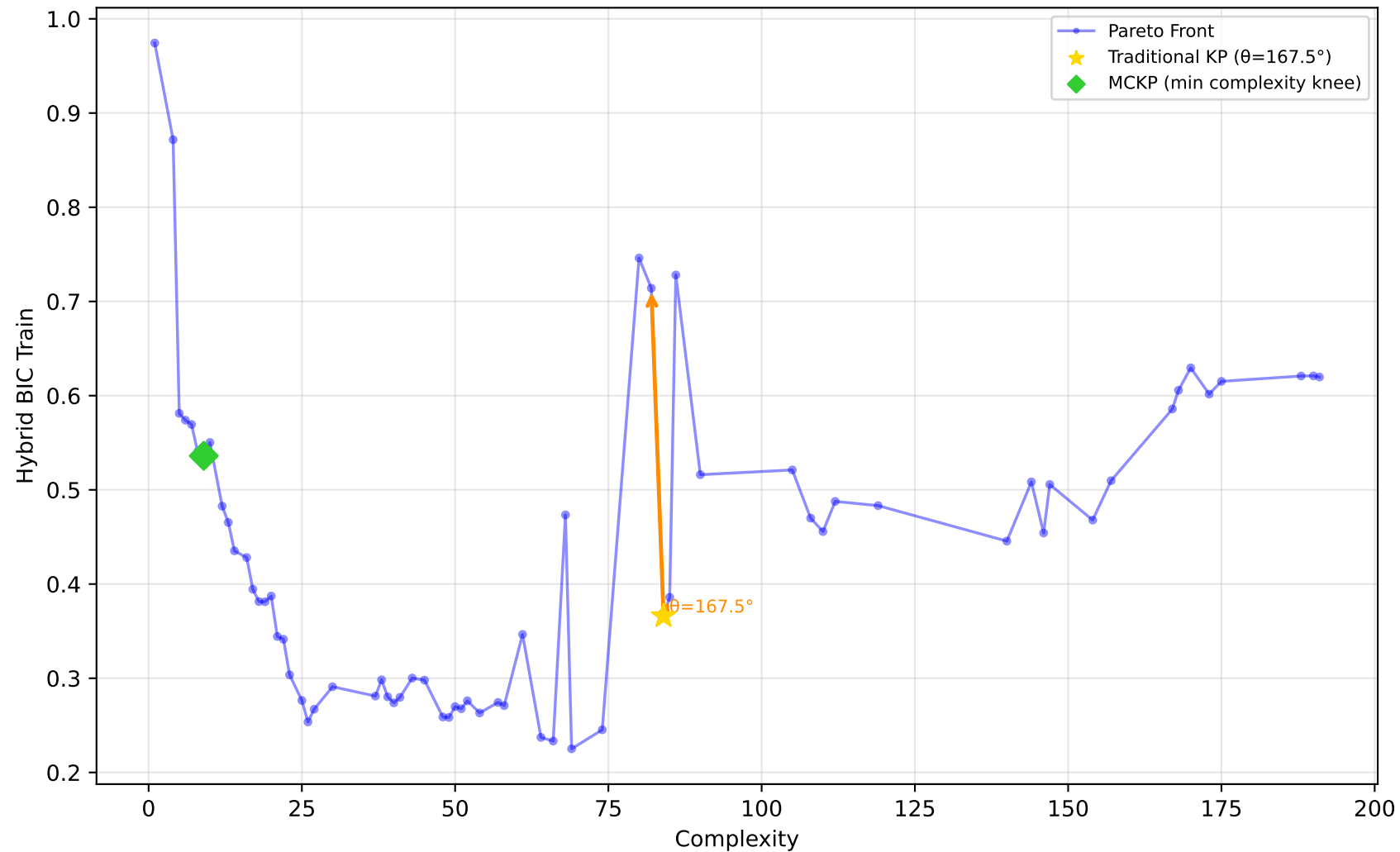
1028_SWD - Run 8 - MVP - Hybrid BIC Train \lambda_1=0.60, \lambda_2=0.00, \lambda_3=0.00 | Difficulty: 1.00 | Method: hmr
