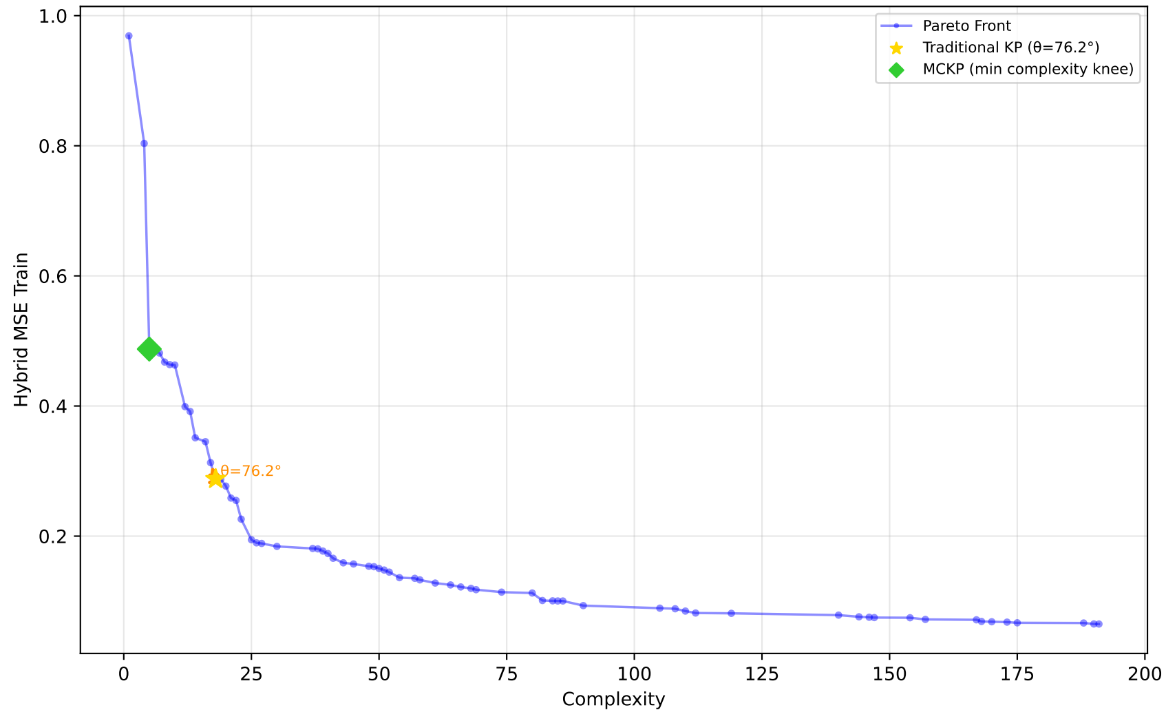
1028_SWD - Run 8 - MVP - Hybrid MSE Train \lambda_1=0.00, \lambda_2=0.00, \lambda_3=0.00 | Difficulty: 1.00 | Method: hmr
