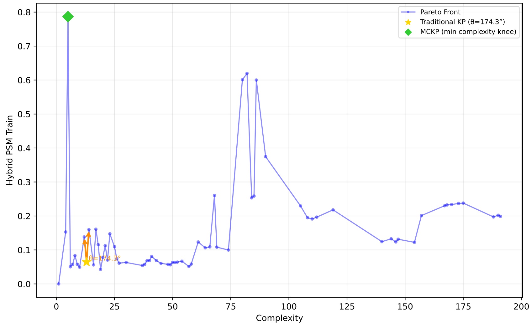
1028_SWD - Run 8 - MVP - Hybrid PSM Train \lambda_1=0.60, \lambda_2=0.00, \lambda_3=0.00 | Difficulty: 1.00 | Method: hmr
