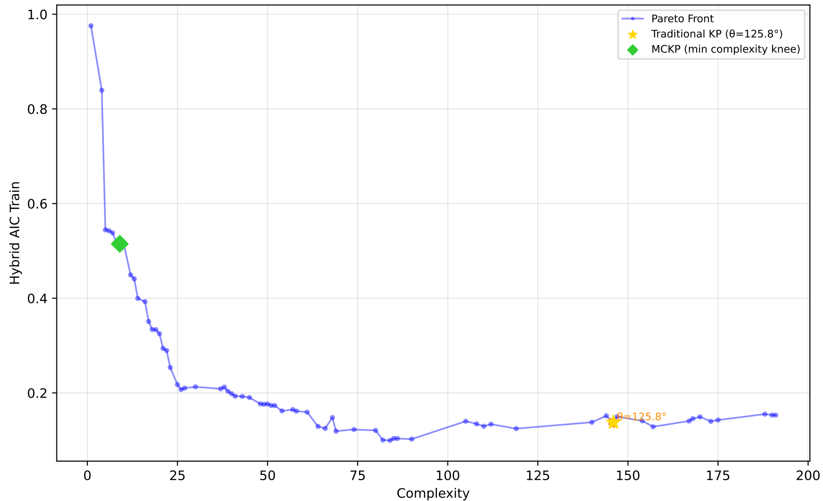
1028_SWD - Run 8 - SVP - Hybrid AIC Train \lambda_1=0.00, \lambda_2=0.60, \lambda_3=0.00 | Difficulty: 1.00 | Method: hmr
