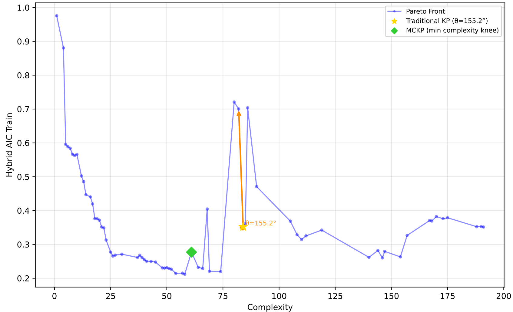
1028_SWD - Run 8 - SVP - Hybrid AIC Train \lambda_1=0.60, \lambda_2=0.00, \lambda_3=0.00 | Difficulty: 1.00 | Method: hmr
