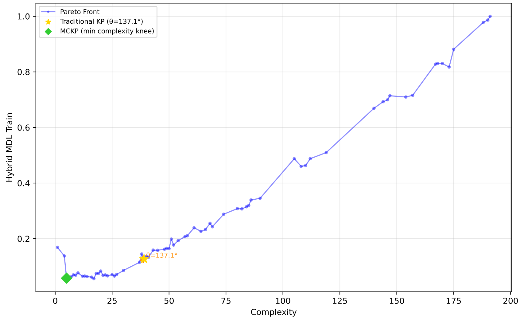
1028_SWD - Run 8 - SVP - Hybrid MDL Train \lambda_1=0.00 , \lambda_2=0.60 , \lambda_3=0.00 | Difficulty: 1.00 | Method: hmr
