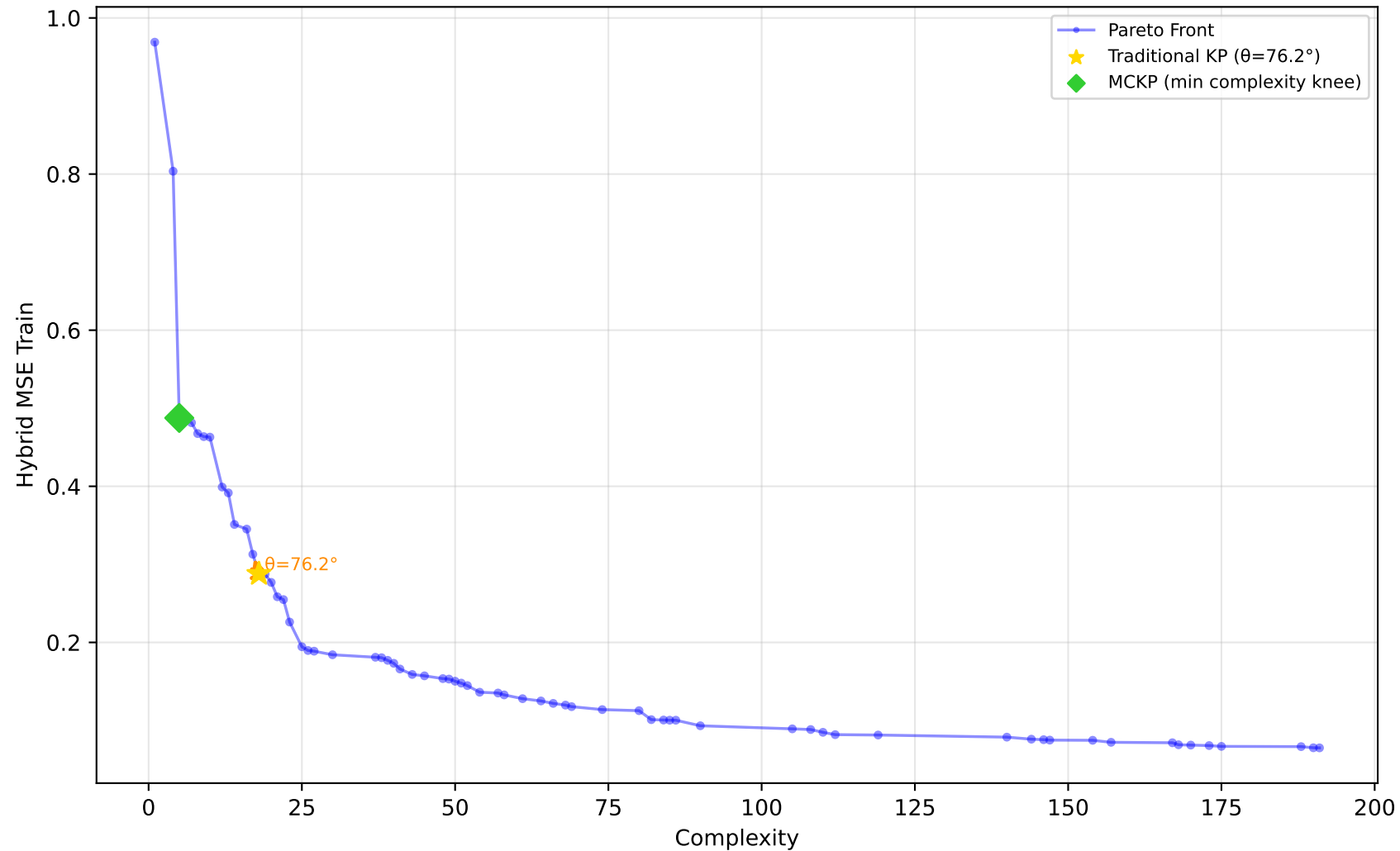
1028_SWD - Run 8 - SVP - Hybrid MSE Train \lambda_1=0.00, \lambda_2=0.60, \lambda_3=0.00 | Difficulty: 1.00 | Method: hmr
