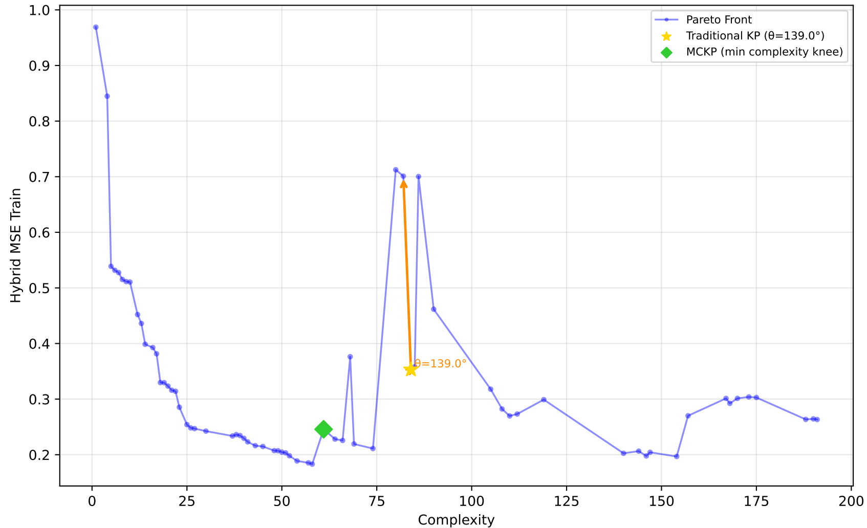
1028_SWD - Run 8 - SVP - Hybrid MSE Train \lambda_1=0.60, \lambda_2=0.00, \lambda_3=0.00 | Difficulty: 1.00 | Method: hmr
