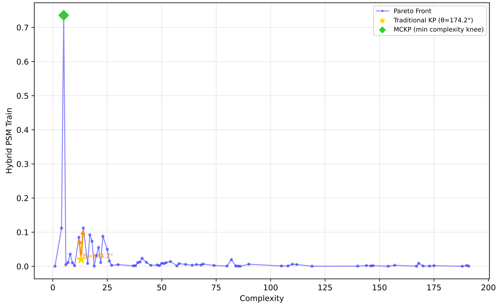
1028_SWD - Run 8 - SVP - Hybrid PSM Train \lambda_1=0.00, \lambda_2=0.60, \lambda_3=0.00 | Difficulty: 1.00 | Method: hmr
