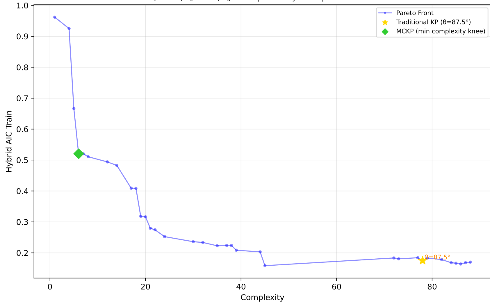
1028_SWD - Run 9 - MVP - Hybrid AIC Train \lambda_1=0.00, \lambda_2=0.00, \lambda_3=0.00 | Difficulty: 1.00 | Method: hmr
