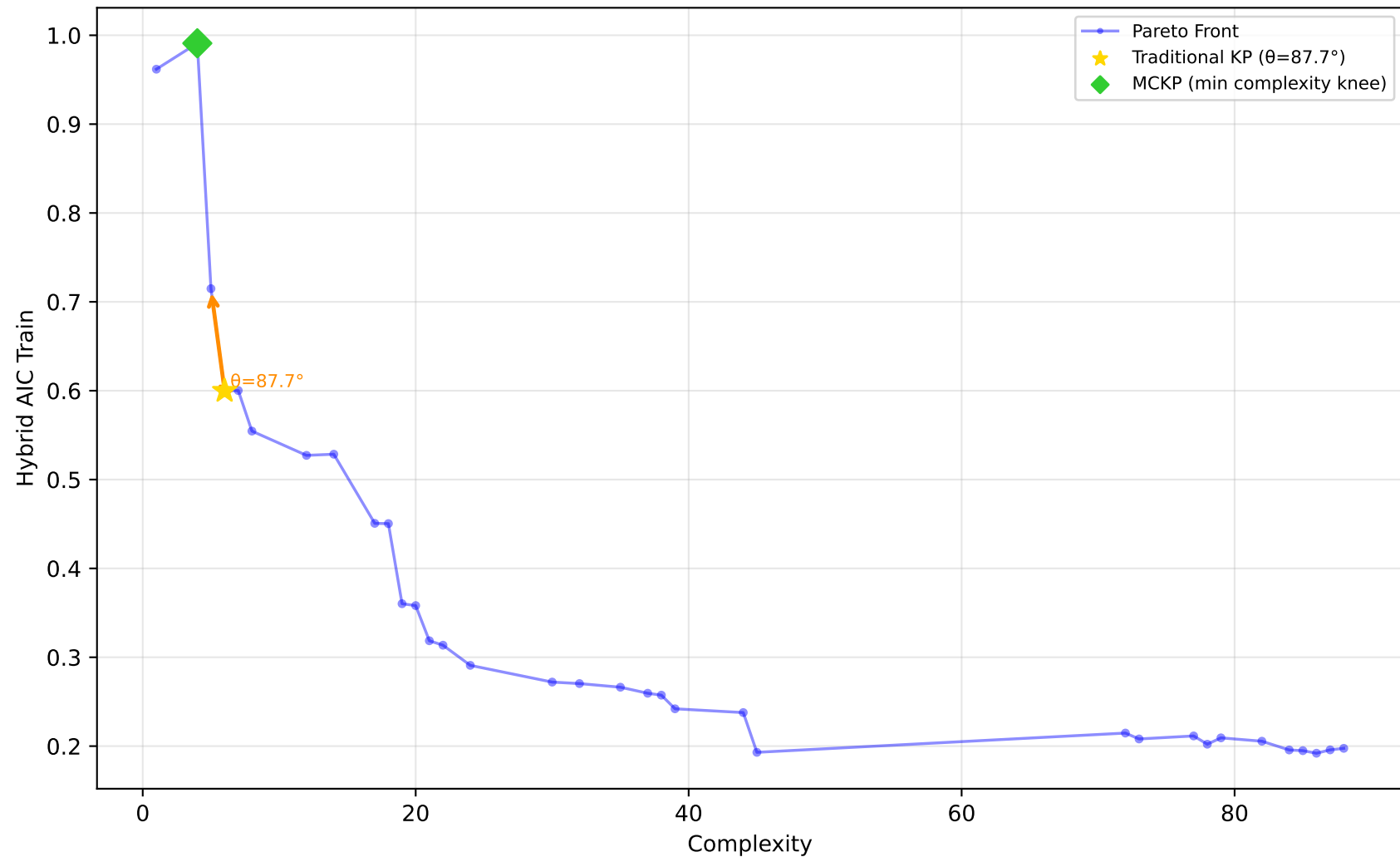
1028_SWD - Run 9 - MVP - Hybrid AIC Train \lambda_1=0.60, \lambda_2=0.00, \lambda_3=0.00 | Difficulty: 1.00 | Method: hmr
