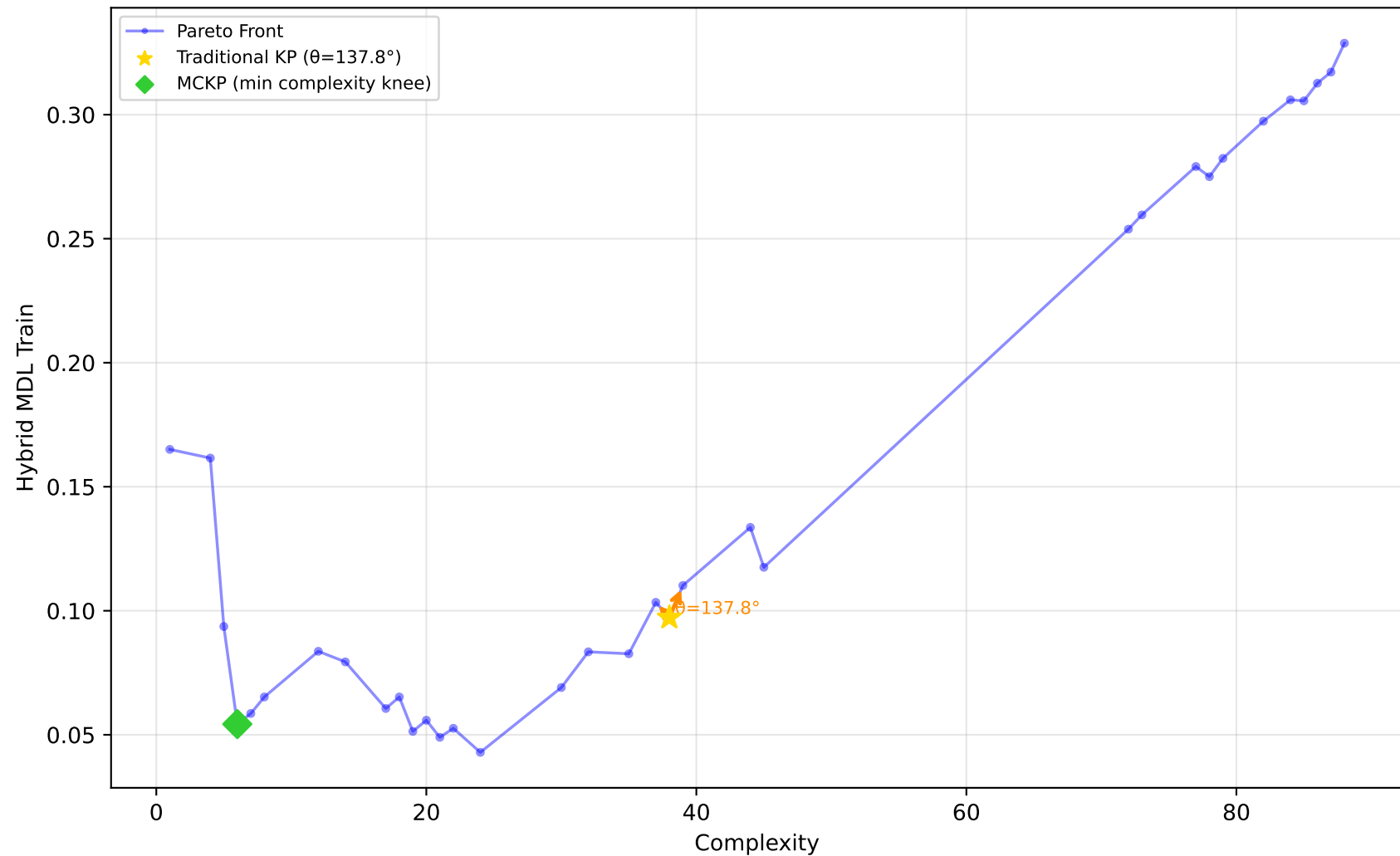
1028_SWD - Run 9 - MVP - Hybrid MDL Train \lambda_1=0.00, \lambda_2=0.00, \lambda_3=0.00 | Difficulty: 1.00 | Method: hmr
