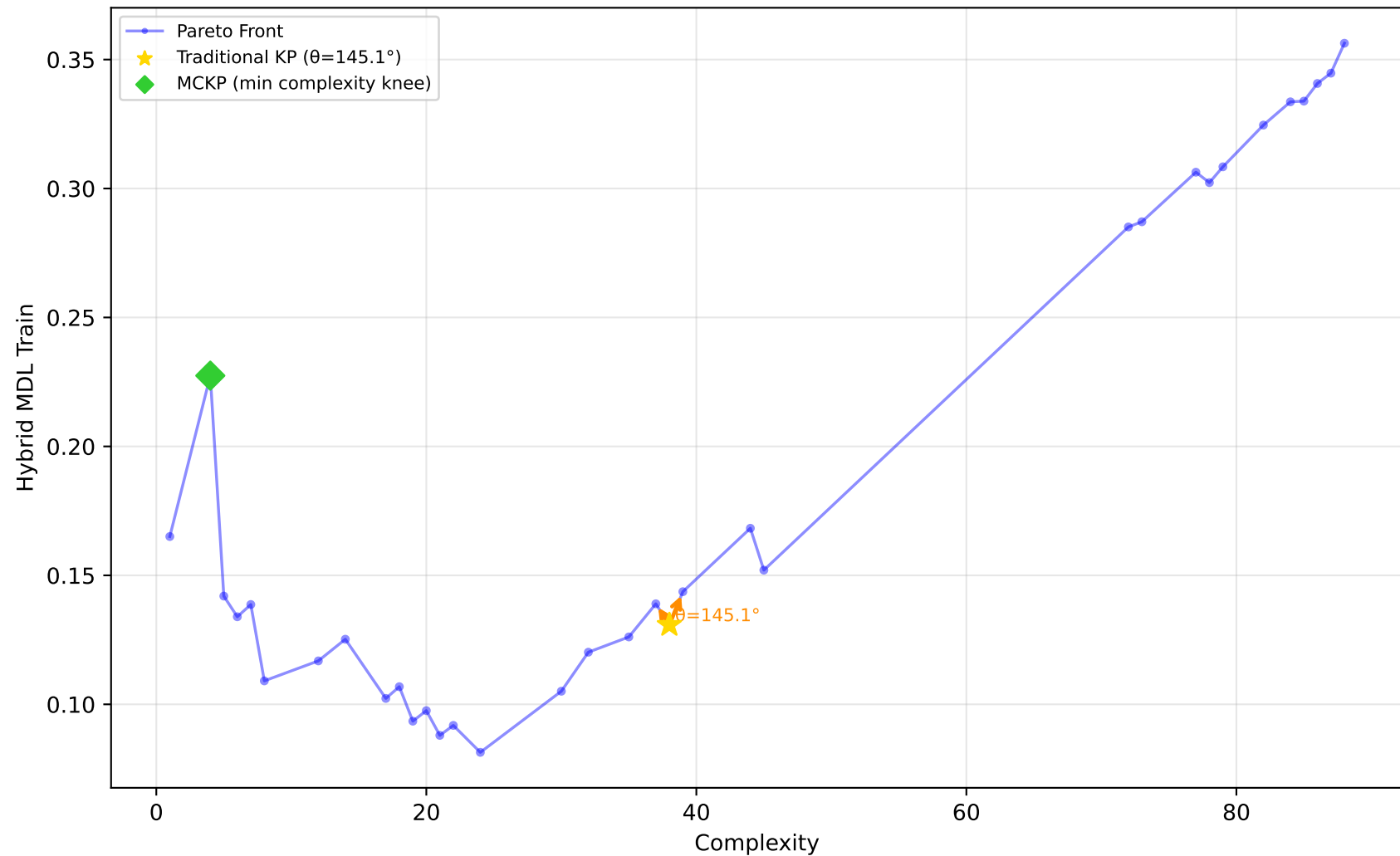
1028_SWD - Run 9 - MVP - Hybrid MDL Train \lambda_1=0.60, \lambda_2=0.00, \lambda_3=0.00 | Difficulty: 1.00 | Method: hmr
