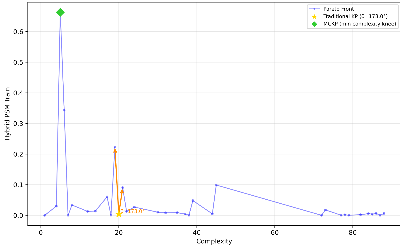
1028_SWD - Run 9 - MVP - Hybrid PSM Train \lambda_1=0.00, \lambda_2=0.00, \lambda_3=0.00 | Difficulty: 1.00 | Method: hmr
