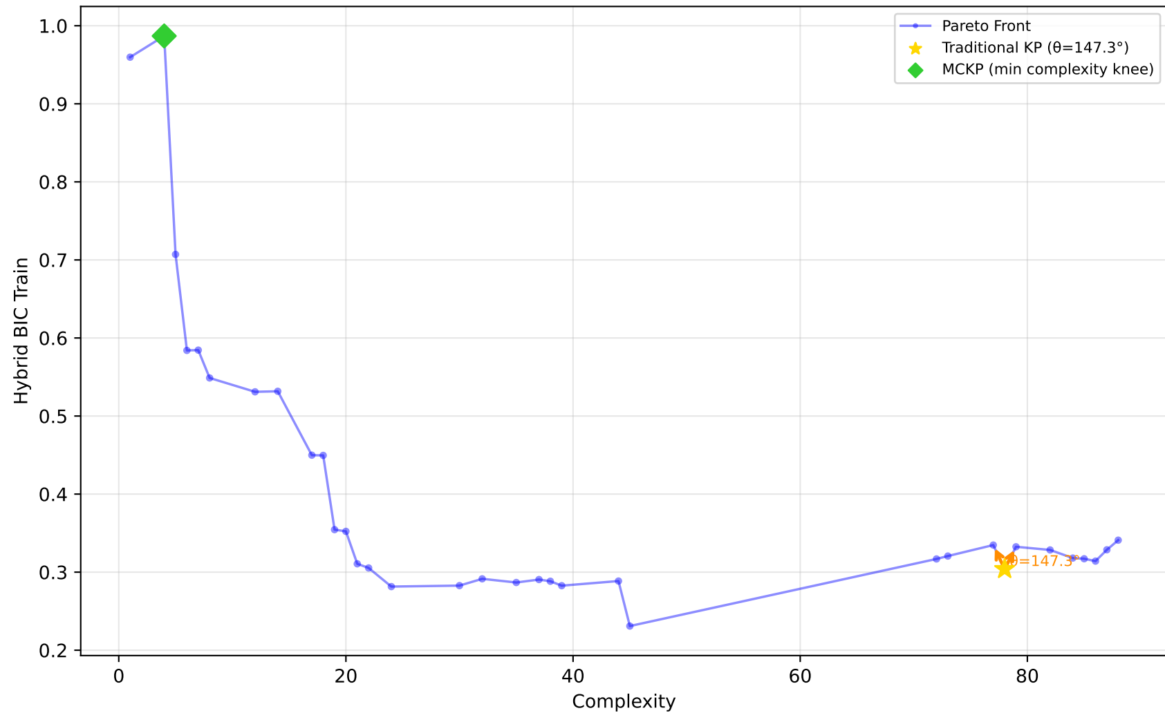
1028_SWD - Run 9 - SVP - Hybrid BIC Train \lambda_1=0.60, \lambda_2=0.00, \lambda_3=0.00 | Difficulty: 1.00 | Method: hmr
