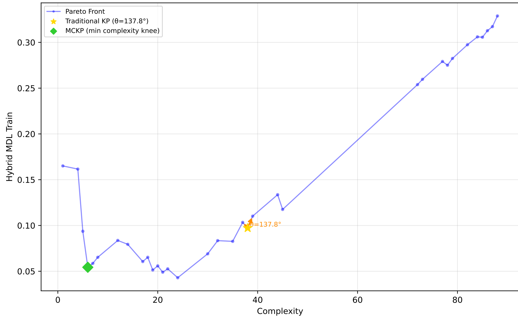
1028_SWD - Run 9 - SVP - Hybrid MDL Train \lambda_1=0.00, \lambda_2=0.60, \lambda_3=0.00 | Difficulty: 1.00 | Method: hmr
