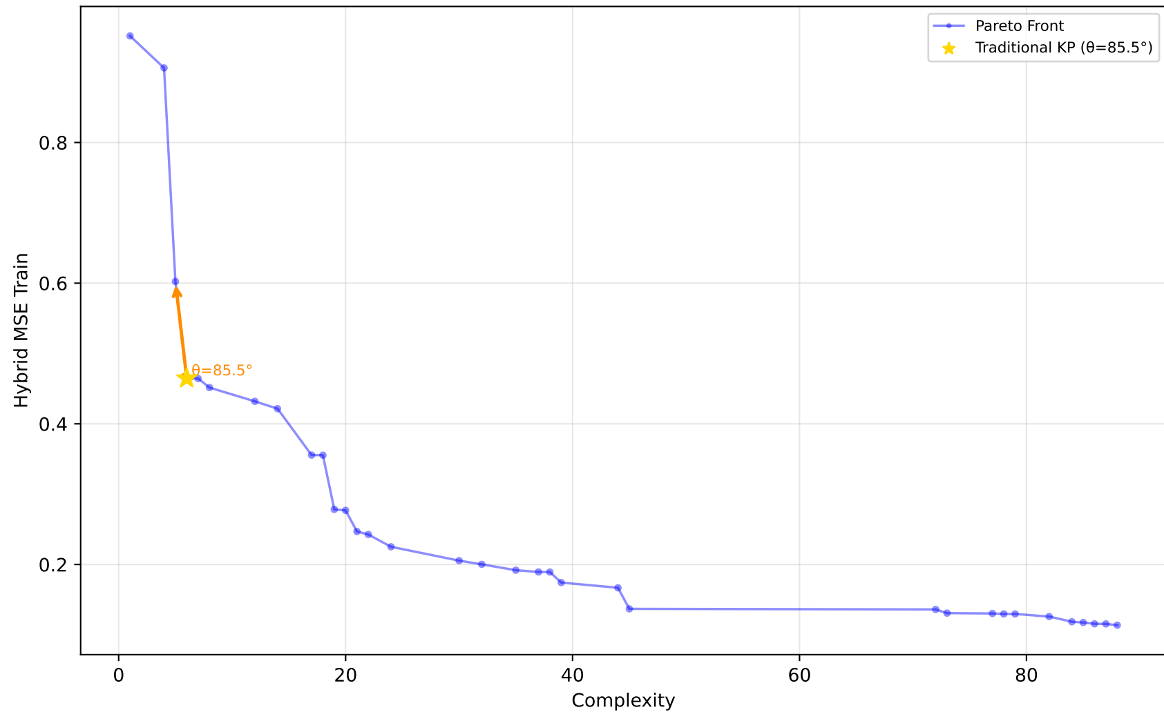
1028_SWD - Run 9 - SVP - Hybrid MSE Train \lambda_1=0.00, \lambda_2=0.60, \lambda_3=0.00 | Difficulty: 1.00 | Method: hmr
