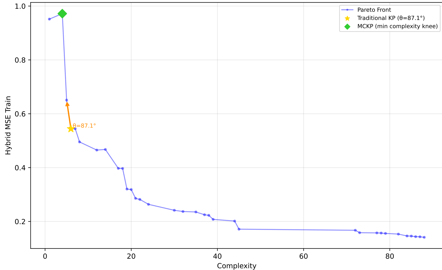
1028_SWD - Run 9 - SVP - Hybrid MSE Train \lambda_1=0.60, \lambda_2=0.00, \lambda_3=0.00 | Difficulty: 1.00 | Method: hmr
