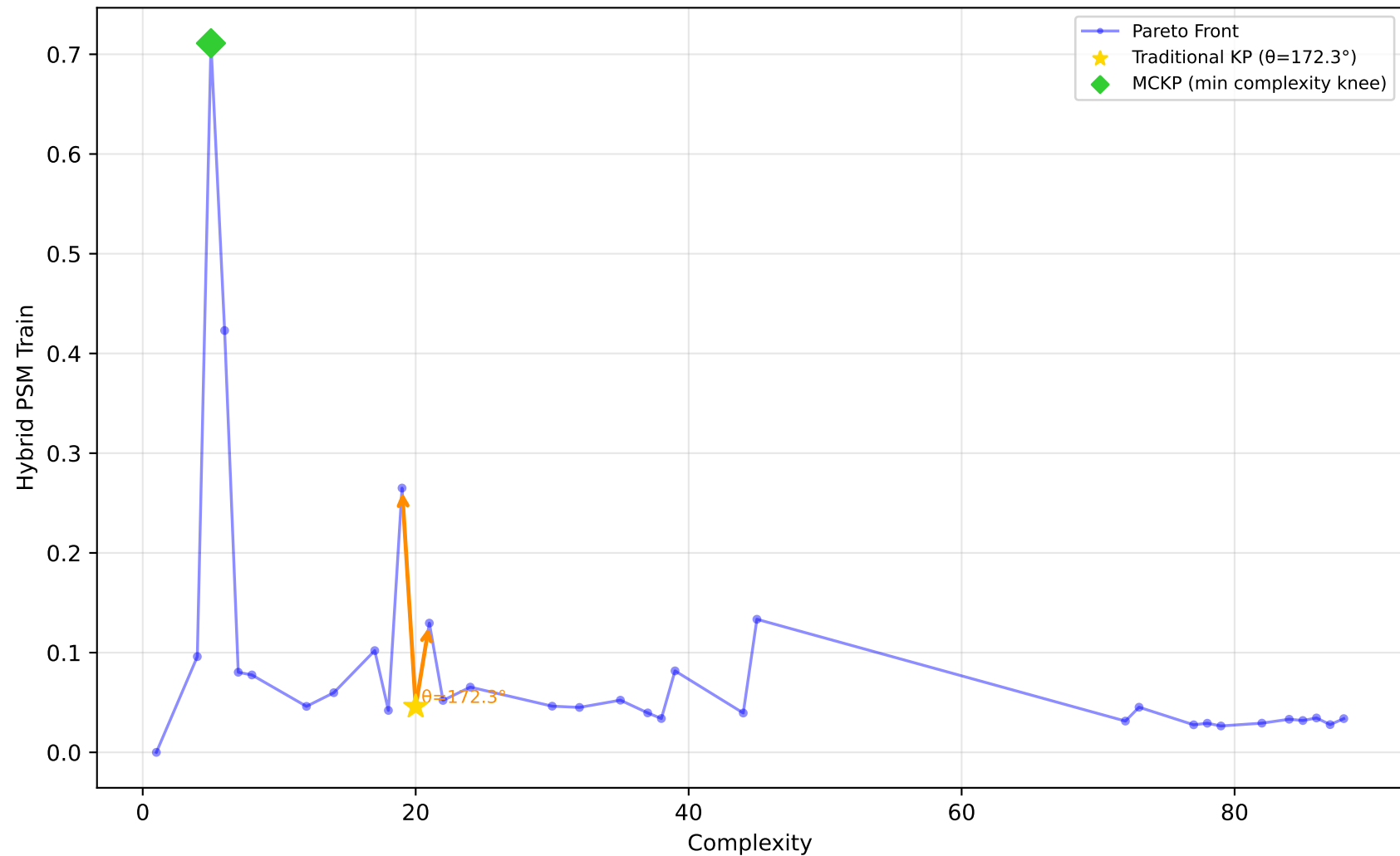
1028_SWD - Run 9 - SVP - Hybrid PSM Train \lambda_1=0.60, \lambda_2=0.00, \lambda_3=0.00 | Difficulty: 1.00 | Method: hmr
