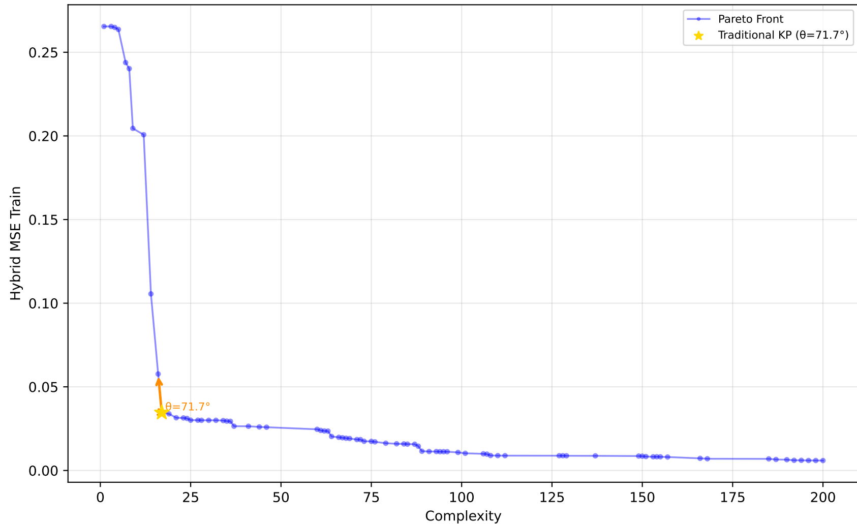
557_analcatdata_apnea1 - Run 10 - MVP - Hybrid MSE Train \lambda_1=0.00, \lambda_2=0.00, \lambda_3=0.00 | Difficulty: 1.00 | Method: hmr
