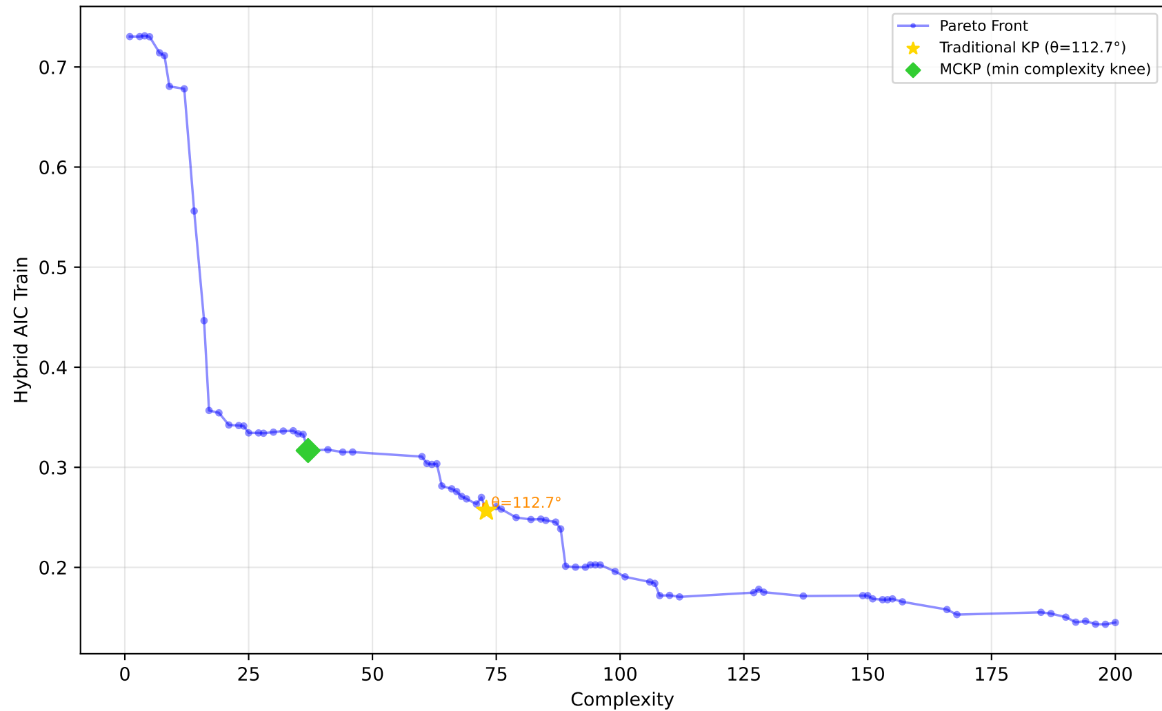
557_analcatdata_apnea1 - Run 10 - SVP - Hybrid AIC Train \lambda_1=0.00 , \lambda_2=0.00 , \lambda_3=0.00 | Difficulty: 1.00 | Method: hmr
