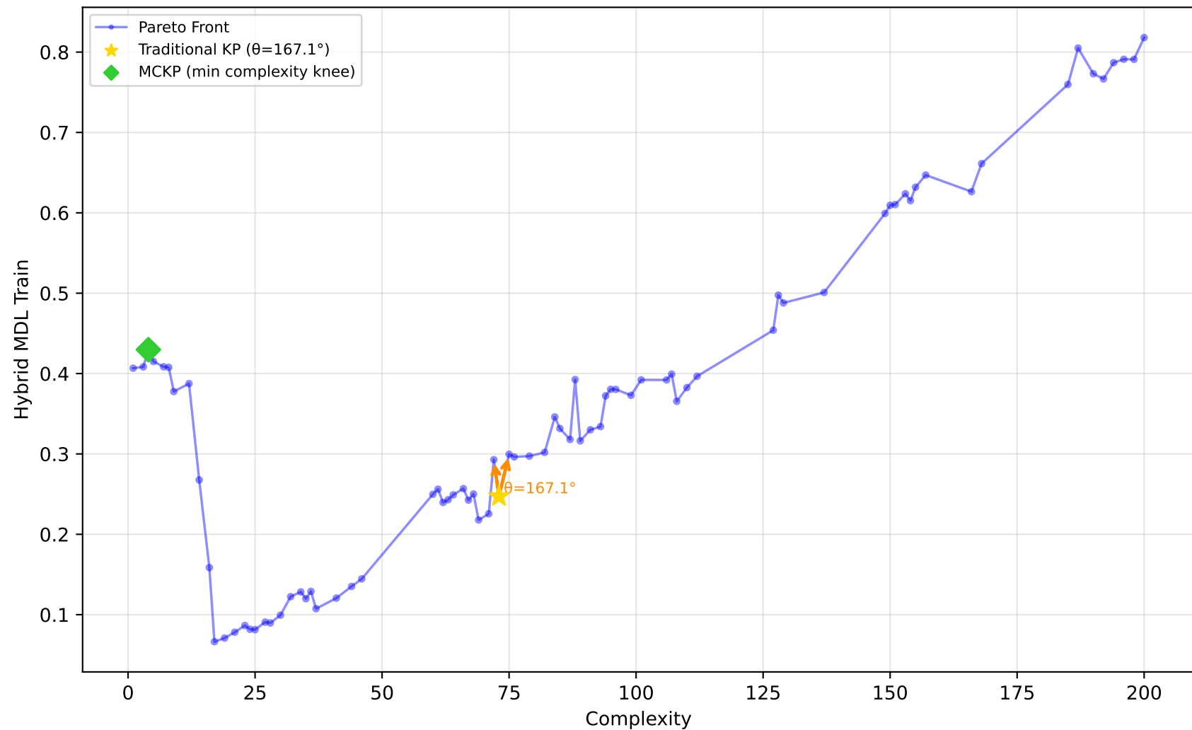
557_analcatdata_apnea1 - Run 10 - SVP - Hybrid MDL Train \lambda_1=0.00, \lambda_2=0.00, \lambda_3=0.00 | Difficulty: 1.00 | Method: hmr
