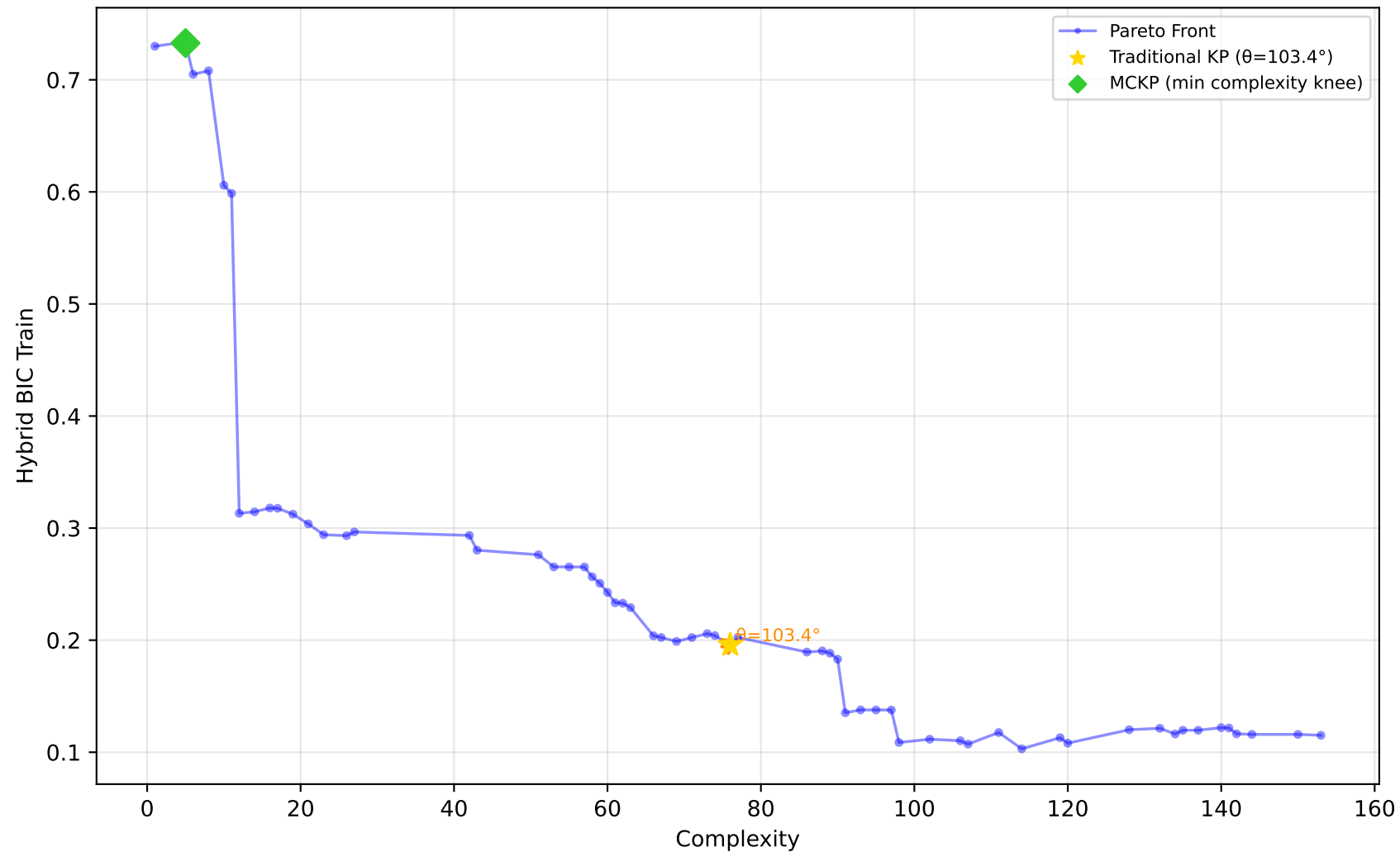
557_analcatdata_apnea1 - Run 11 - MVP - Hybrid BIC Train \lambda_1=0.00, \lambda_2=0.00, \lambda_3=0.00 | Difficulty: 1.00 | Method: hmr
