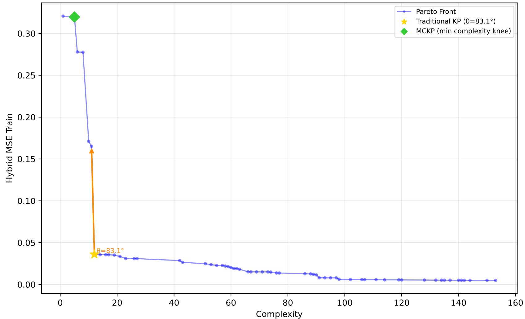
557_analcatdata_apnea1 - Run 11 - MVP - Hybrid MSE Train \lambda_1=0.00, \lambda_2=0.00, \lambda_3=0.00 | Difficulty: 1.00 | Method: hmr
