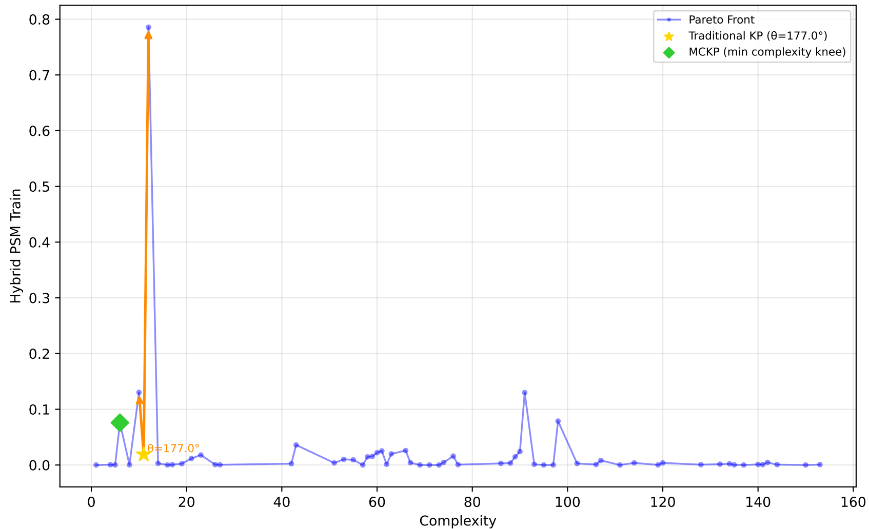
557_analcatdata_apnea1 - Run 11 - SVP - Hybrid PSM Train \lambda_1=0.00, \lambda_2=0.00, \lambda_3=0.00 | Difficulty: 1.00 | Method: hmr
