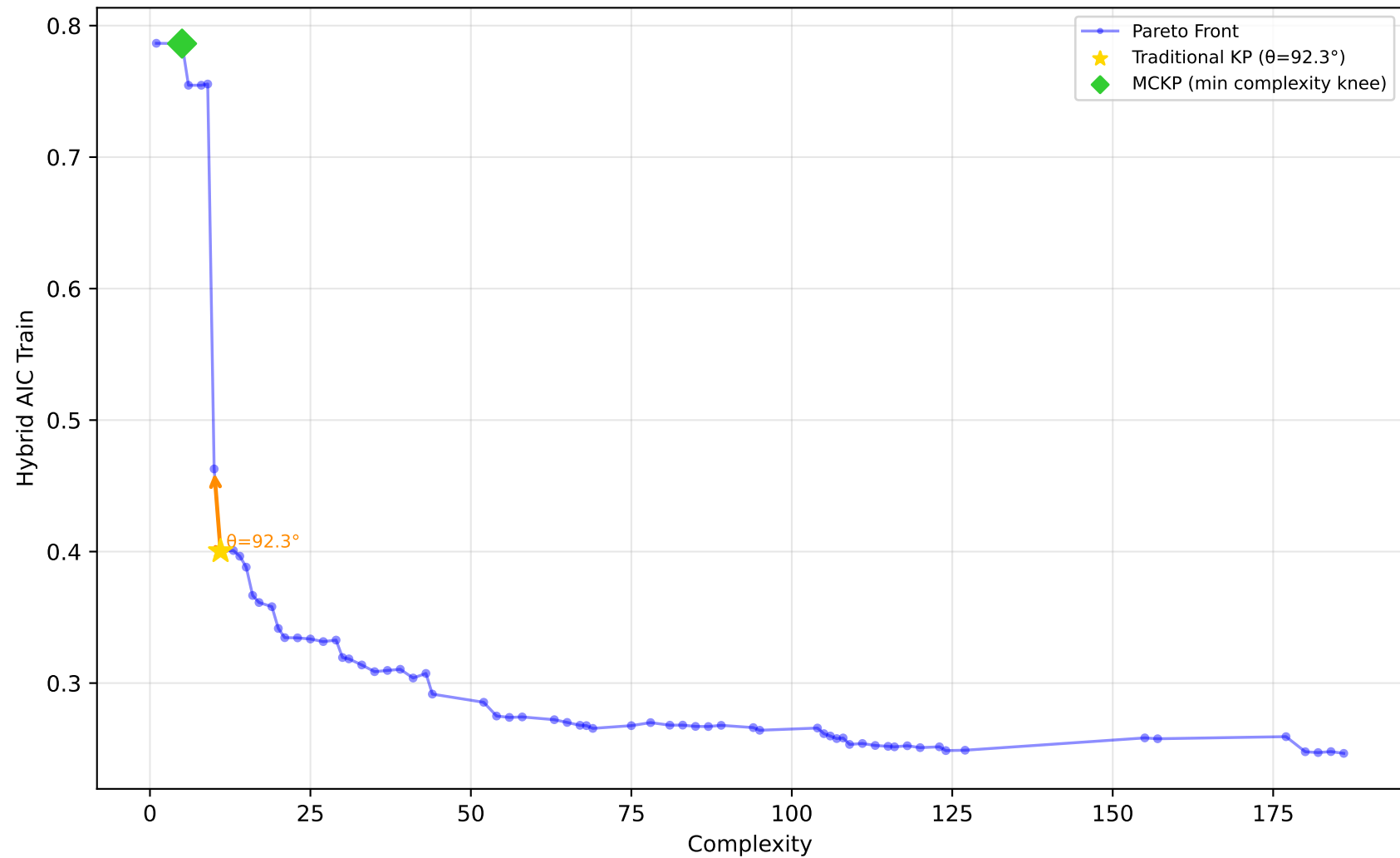
557_analcatdata_apnea1 - Run 12 - MVP - Hybrid AIC Train \lambda_1=0.00, \lambda_2=0.00, \lambda_3=0.00 | Difficulty: 1.00 | Method: hmr
