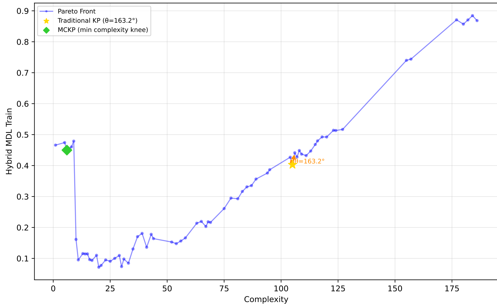
557_analcatdata_apnea1 - Run 12 - MVP - Hybrid MDL Train \lambda_1=0.00, \lambda_2=0.00, \lambda_3=0.00 | Difficulty: 1.00 | Method: hmr
