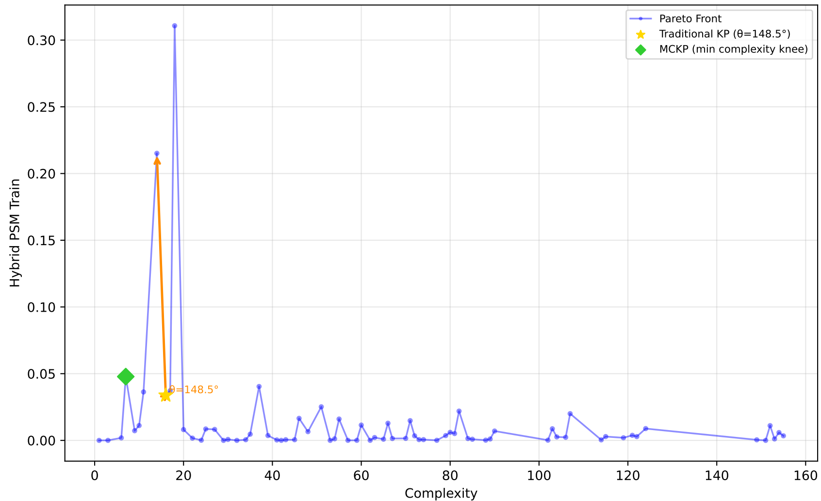
557_analcatdata_apnea1 - Run 13 - MVP - Hybrid PSM Train \lambda_1=0.00 , \lambda_2=0.00 , \lambda_3=0.00 | Difficulty: 0.95 | Method: hmr
