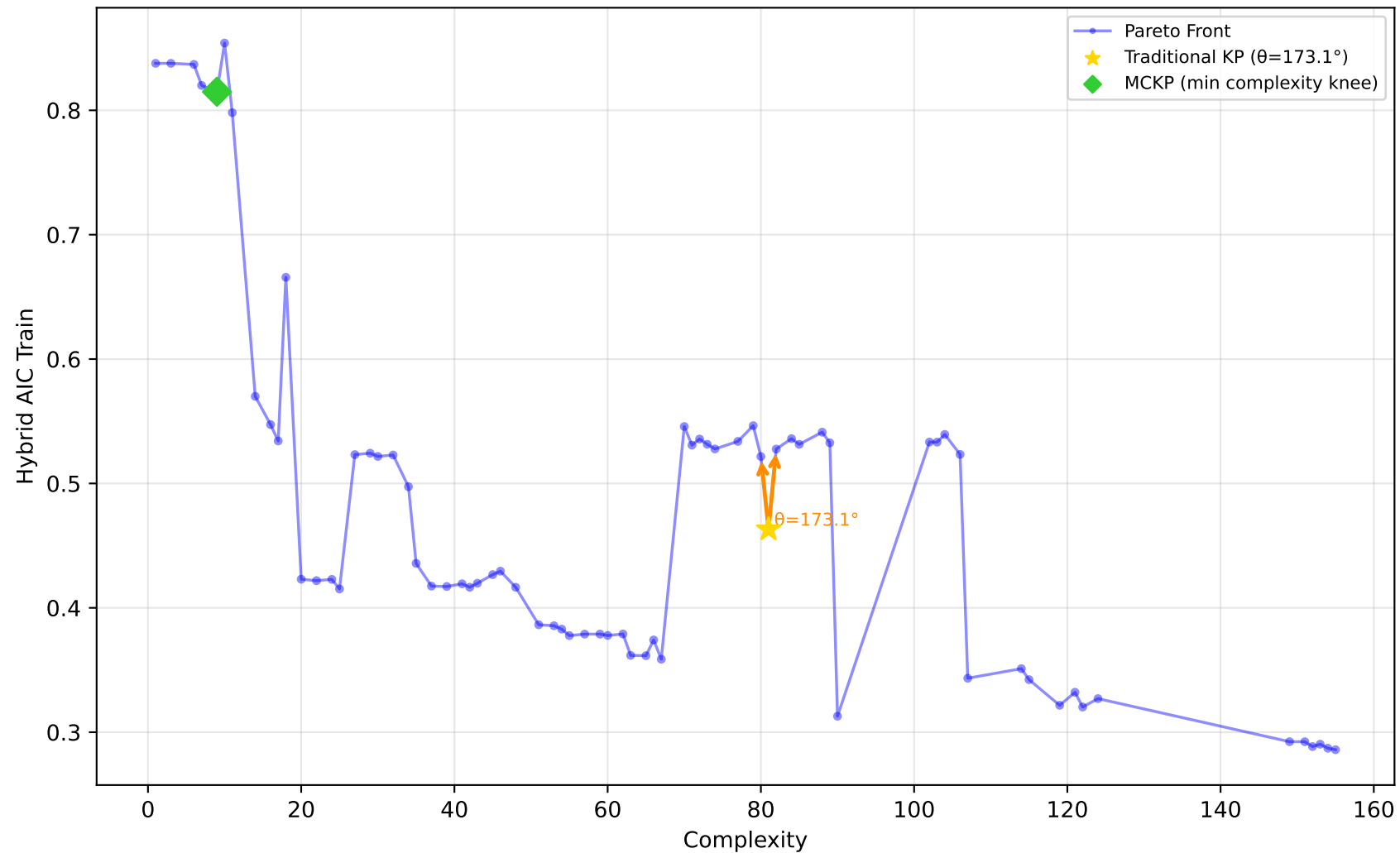
557_analcatdata_apnea1 - Run 13 - SVP - Hybrid AIC Train \lambda_1=0.00, \lambda_2=0.00, \lambda_3=0.00 | Difficulty: 0.95 | Method: hmr
