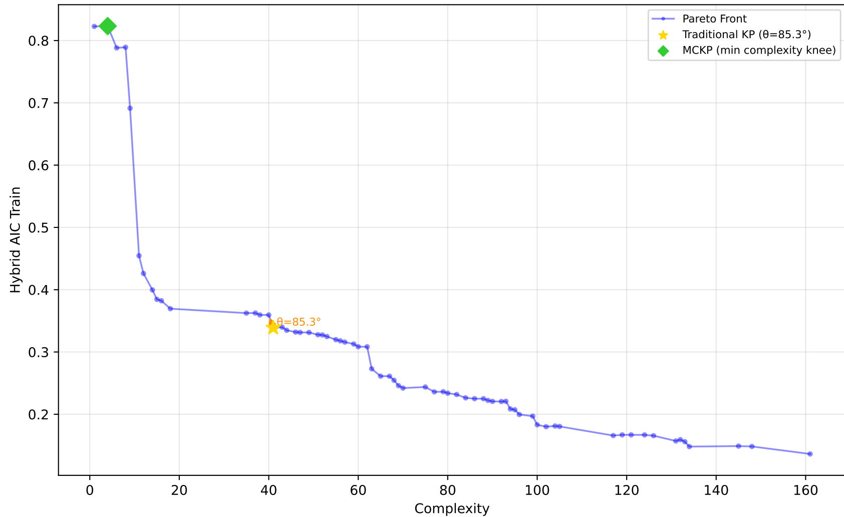
557_analcatdata_apnea1 - Run 14 - SVP - Hybrid AIC Train \lambda_1=0.00, \lambda_2=0.00, \lambda_3=0.00 | Difficulty: 0.63 | Method: hmr
