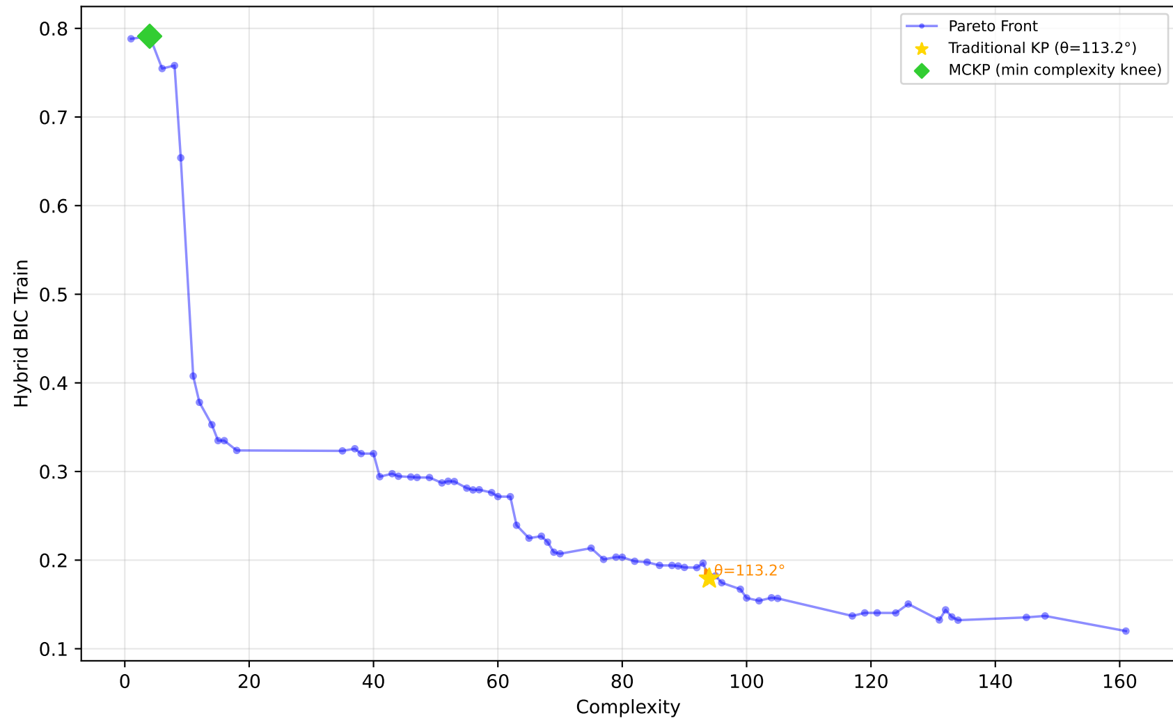
557_analcatdata_apnea1 - Run 14 - SVP - Hybrid BIC Train \lambda_1=0.00, \lambda_2=0.00, \lambda_3=0.00 | Difficulty: 0.63 | Method: hmr
