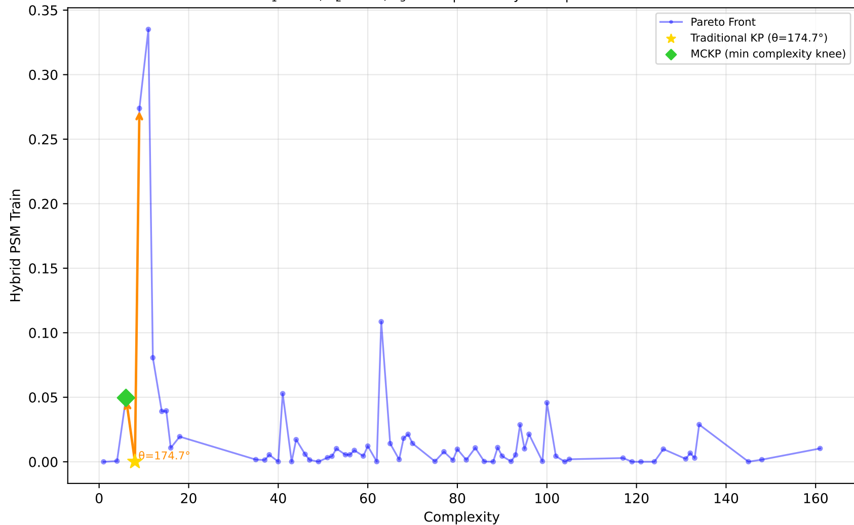
557_analcatdata_apnea1 - Run 14 - SVP - Hybrid PSM Train \lambda_1=0.00 , \lambda_2=0.00 , \lambda_3=0.00 | Difficulty: 0.63 | Method: hmr
