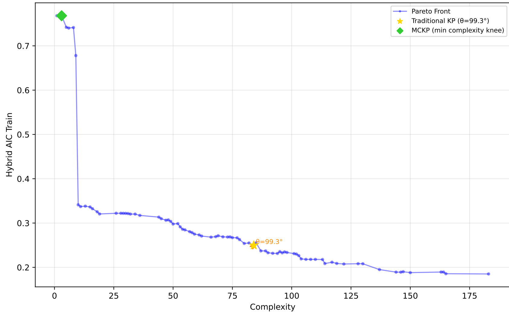
557_analcatdata_apnea1 - Run 15 - SVP - Hybrid AIC Train \lambda_1=0.00, \lambda_2=0.00, \lambda_3=0.00 | Difficulty: 1.00 | Method: hmr
