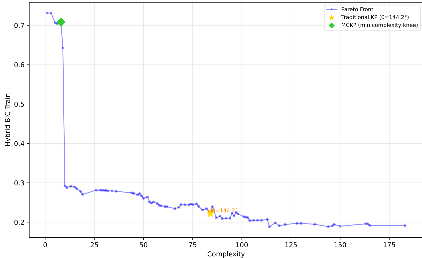
557_analcatdata_apnea1 - Run 15 - SVP - Hybrid BIC Train \lambda_1=0.00, \lambda_2=0.00, \lambda_3=0.00 | Difficulty: 1.00 | Method: hmr
