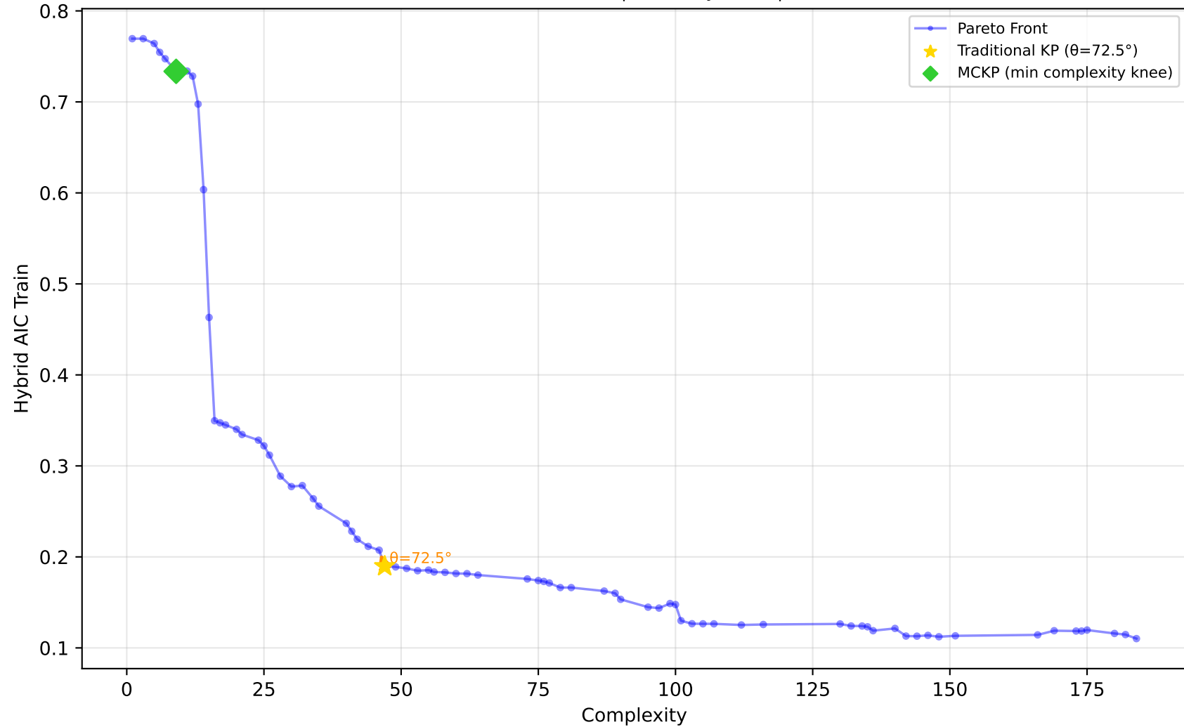
557_analcatdata_apnea1 - Run 16 - SVP - Hybrid AIC Train \lambda_1=0.00, \lambda_2=0.00, \lambda_3=0.00 | Difficulty: 1.00 | Method: hmr
