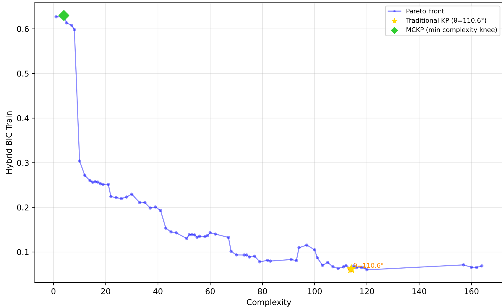
557_analcatdata_apnea1 - Run 17 - MVP - Hybrid BIC Train \lambda_1=0.00, \lambda_2=0.00, \lambda_3=0.00 | Difficulty: 1.00 | Method: hmr
