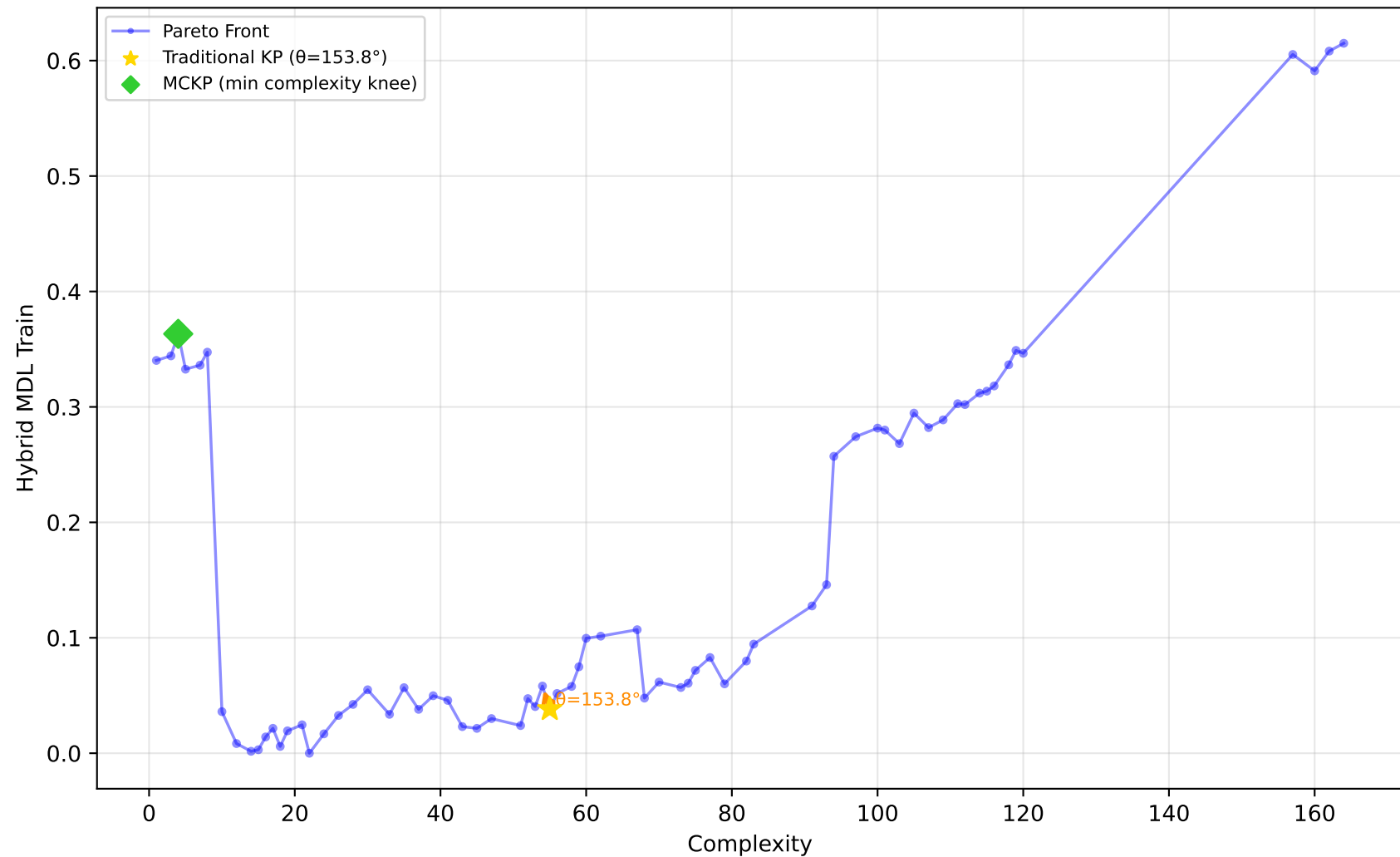
557_analcatdata_apnea1 - Run 17 - SVP - Hybrid MDL Train \lambda_1=0.00, \lambda_2=0.00, \lambda_3=0.00 | Difficulty: 1.00 | Method: hmr
