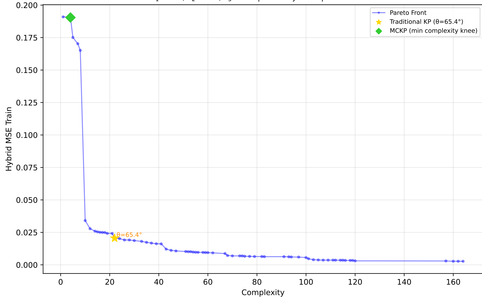
557_analcatdata_apnea1 - Run 17 - SVP - Hybrid MSE Train \lambda_1=0.00 , \lambda_2=0.00 , \lambda_3=0.00 | Difficulty: 1.00 | Method: hmr
