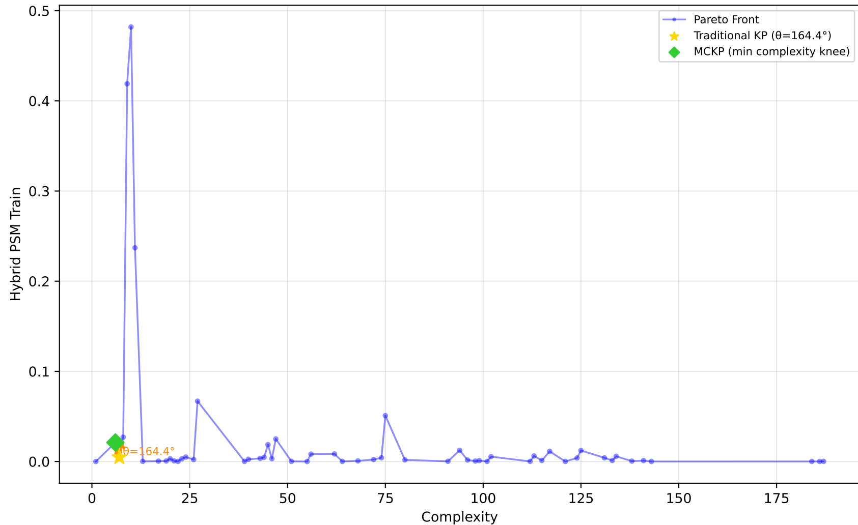
557_analcatdata_apnea1 - Run 18 - MVP - Hybrid PSM Train \lambda_1=0.00, \lambda_2=0.00, \lambda_3=0.00 | Difficulty: 1.00 | Method: hmr
