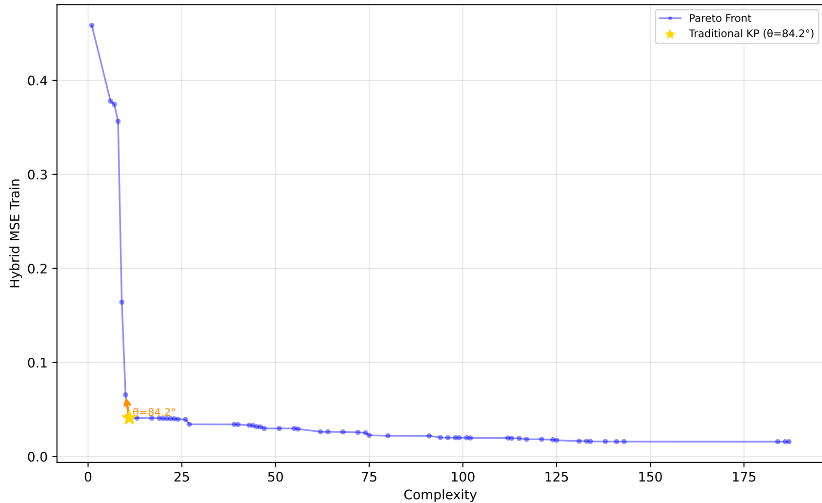
557_analcatdata_apnea1 - Run 18 - SVP - Hybrid MSE Train \lambda_1=0.00 , \lambda_2=0.00 , \lambda_3=0.00 | Difficulty: 1.00 | Method: hmr
