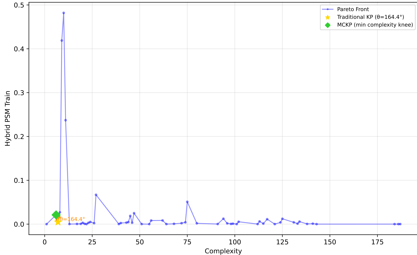
557_analcatdata_apnea1 - Run 18 - SVP - Hybrid PSM Train \lambda_1=0.00, \lambda_2=0.00, \lambda_3=0.00 | Difficulty: 1.00 | Method: hmr
