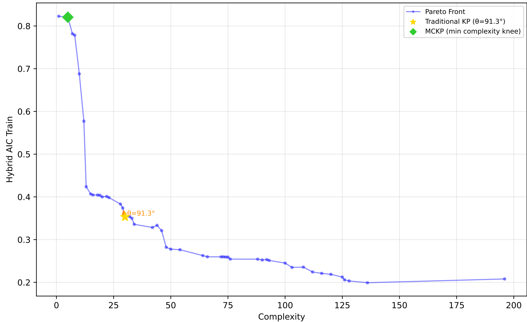
557_analcatdata_apnea1 - Run 19 - MVP - Hybrid AIC Train \lambda_1=0.00, \lambda_2=0.00, \lambda_3=0.00 | Difficulty: 1.00 | Method: hmr
