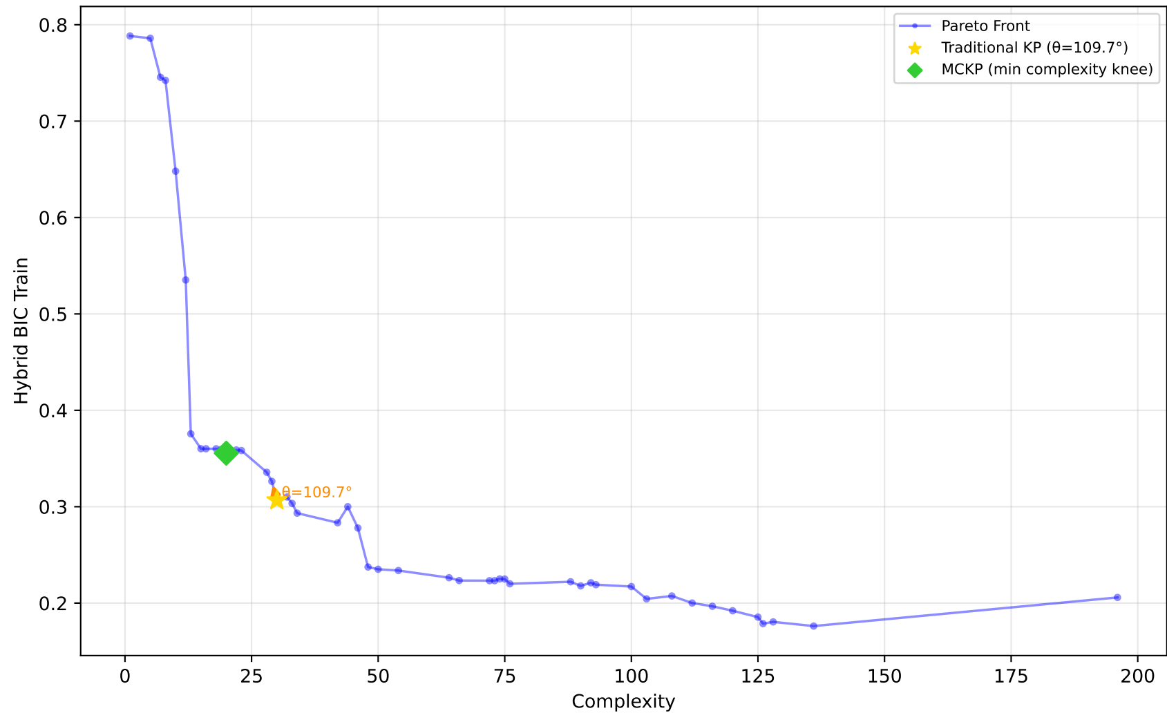
557_analcatdata_apnea1 - Run 19 - MVP - Hybrid BIC Train \lambda_1=0.00, \lambda_2=0.00, \lambda_3=0.00 | Difficulty: 1.00 | Method: hmr
