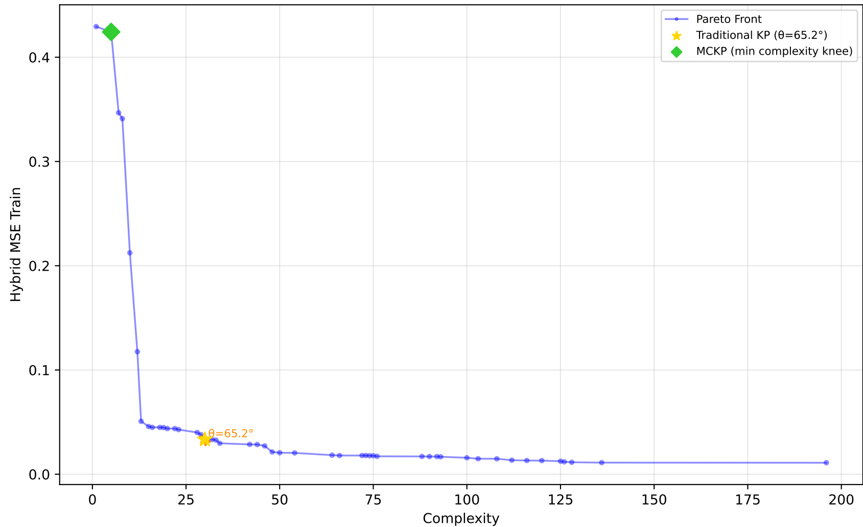
557_analcatdata_apnea1 - Run 19 - MVP - Hybrid MSE Train \lambda_1=0.00, \lambda_2=0.00, \lambda_3=0.00 | Difficulty: 1.00 | Method: hmr
