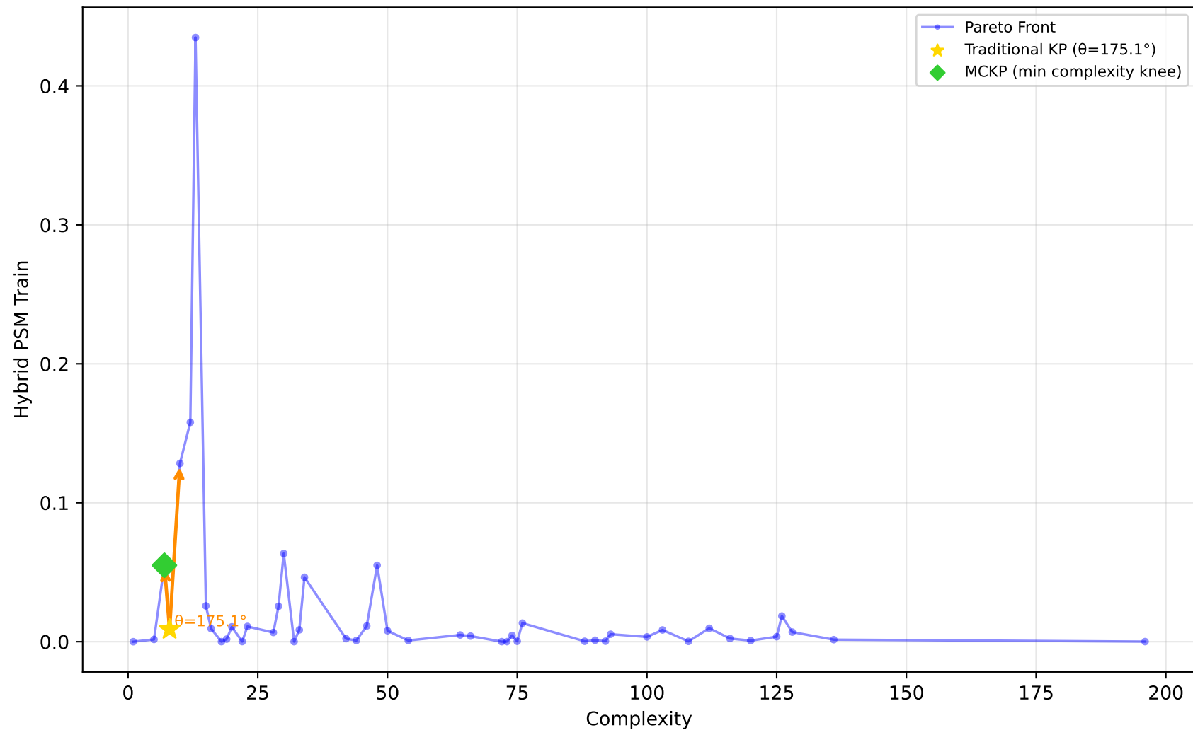
557_analcatdata_apnea1 - Run 19 - MVP - Hybrid PSM Train \lambda_1=0.00, \lambda_2=0.00, \lambda_3=0.00 | Difficulty: 1.00 | Method: hmr
