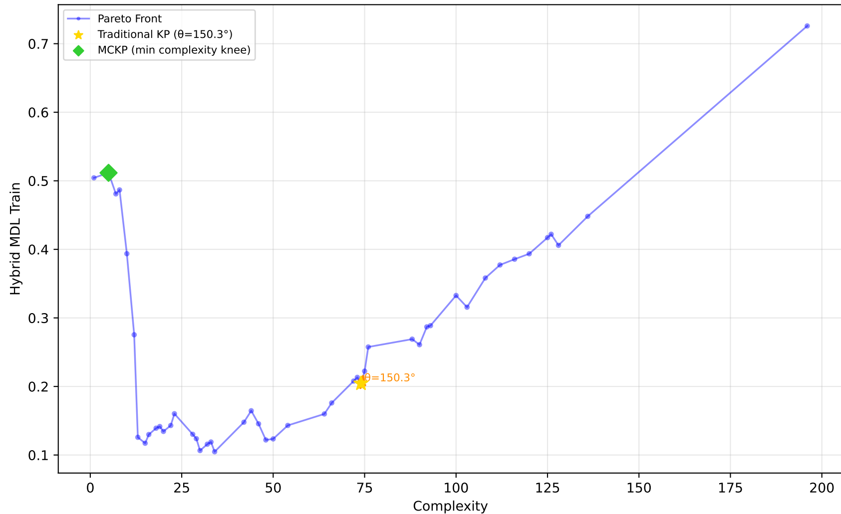
557_analcatdata_apnea1 - Run 19 - SVP - Hybrid MDL Train \lambda_1=0.00, \lambda_2=0.00, \lambda_3=0.00 | Difficulty: 1.00 | Method: hmr
