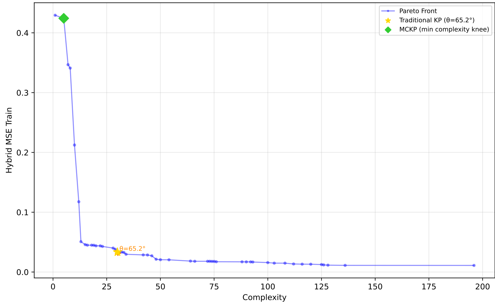
557_analcatdata_apnea1 - Run 19 - SVP - Hybrid MSE Train \lambda_1=0.00, \lambda_2=0.00, \lambda_3=0.00 | Difficulty: 1.00 | Method: hmr
