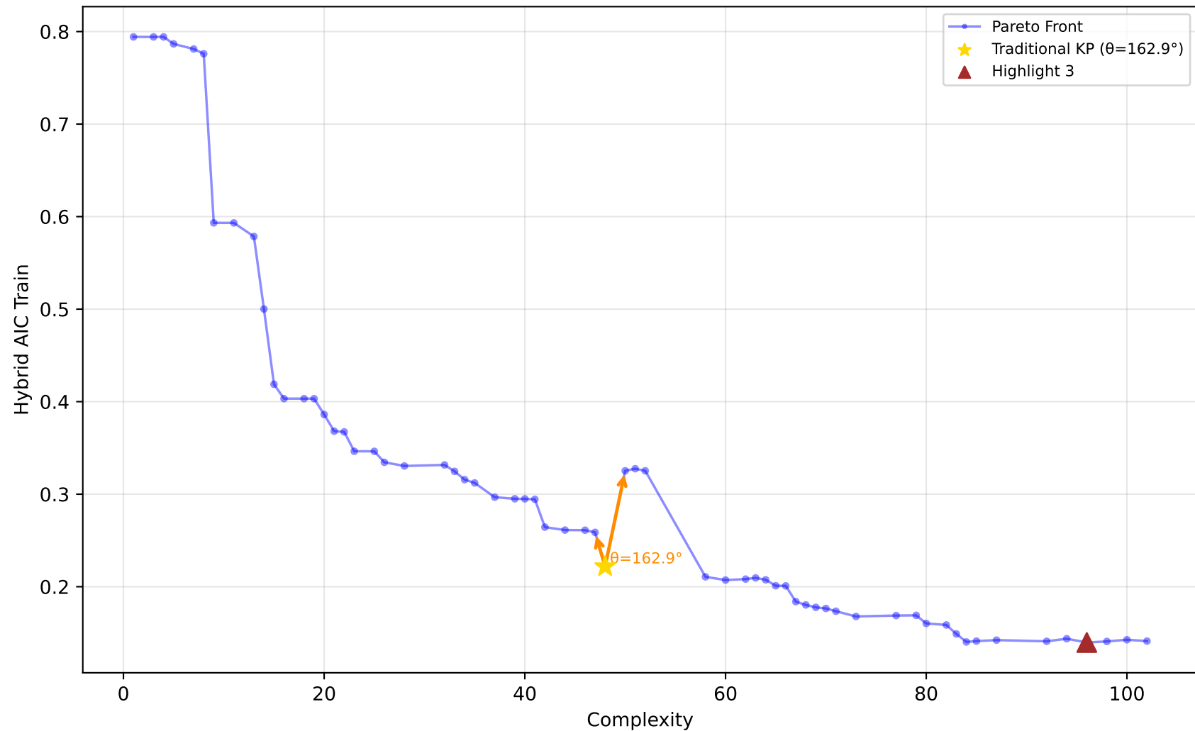
557_analcatdata_apnea1 - Run 1 - MVP - Hybrid AIC Train \lambda_1=0.00, \lambda_2=0.00, \lambda_3=0.00 | Difficulty: 1.00 | Method: hmr
