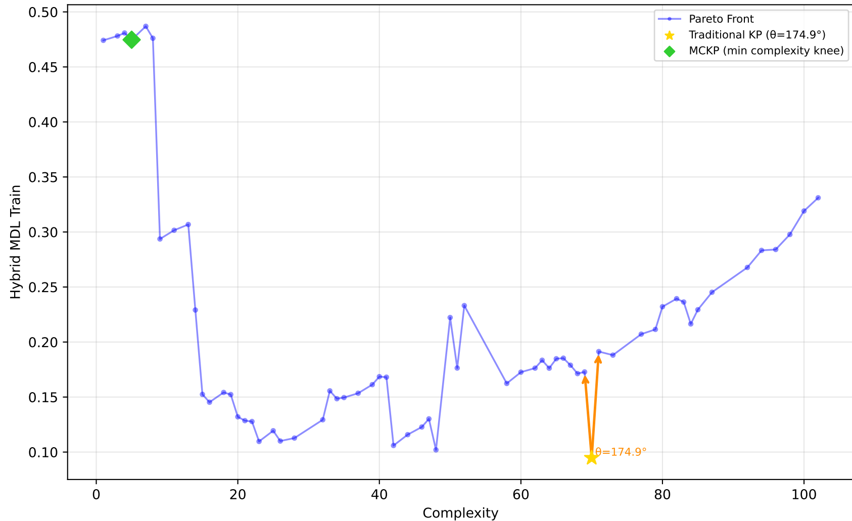
557_analcatdata_apnea1 - Run 1 - MVP - Hybrid MDL Train \lambda_1=0.00, \lambda_2=0.00, \lambda_3=0.00 | Difficulty: 1.00 | Method: hmr
