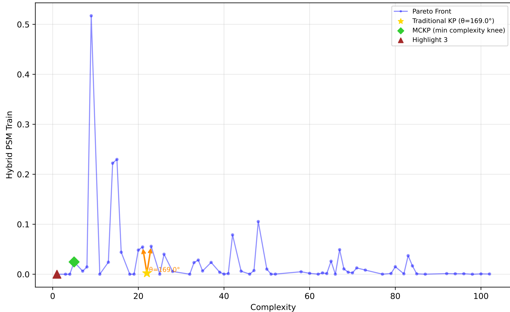
557_analcatdata_apnea1 - Run 1 - MVP - Hybrid PSM Train \lambda_1=0.00, \lambda_2=0.00, \lambda_3=0.00 | Difficulty: 1.00 | Method: hmr
